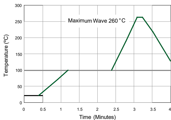
Lead-free Profile
